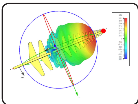
Radiation Pattern at 1710 MHz
