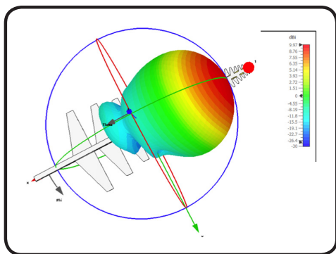
Radiation Pattern at 700 MHz
