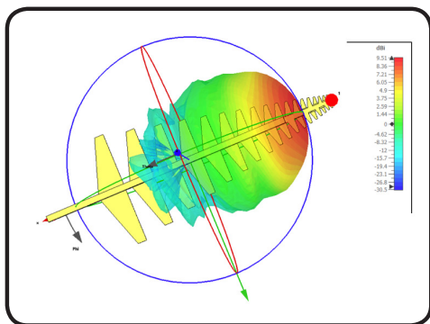
Radiation Pattern at 2300 MHz
