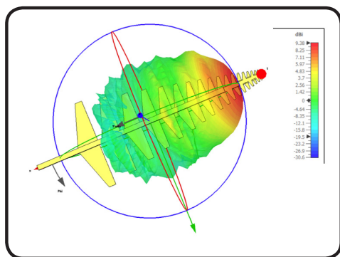
Radiation Pattern at 3600 MHz
