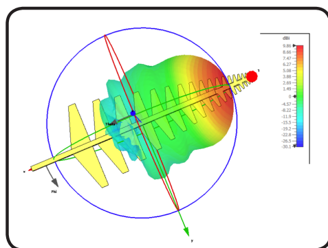
Radiation Pattern at 1880 MHz
