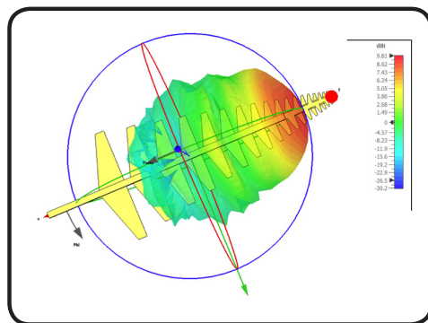
Radiation Pattern at 2700 MHz
