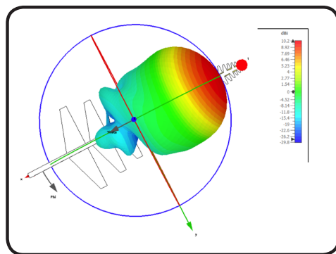
Radiation Pattern at 960 MHz
